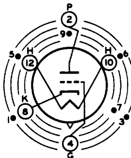
TERMINAL DIAGRAM Bottom View
